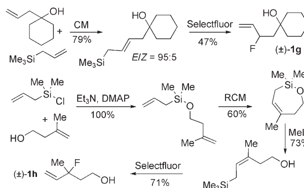
Scheme 1. Synthesis of allylic fluorides ( \pm )- 1g and ( \pm )- 1h .
